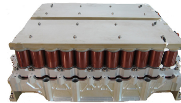
VES16 11s16p battery
