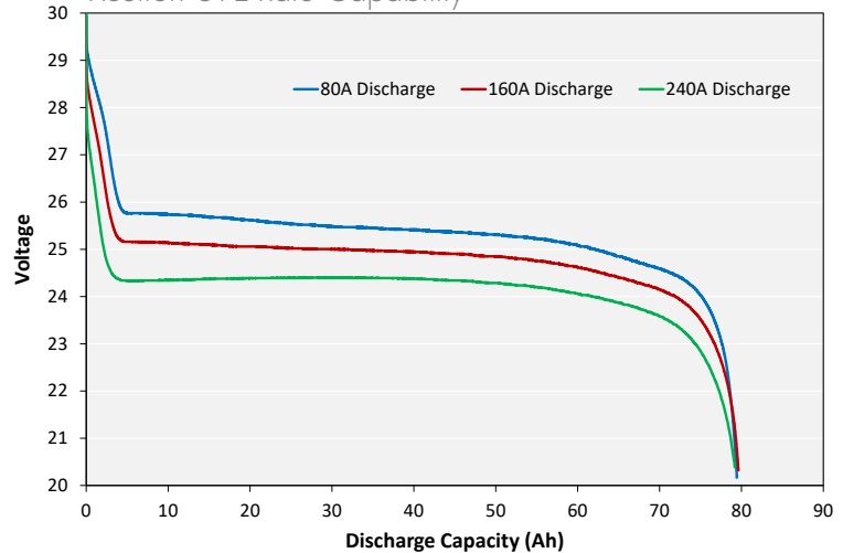
Xcelion 6T-E Rate Capability
