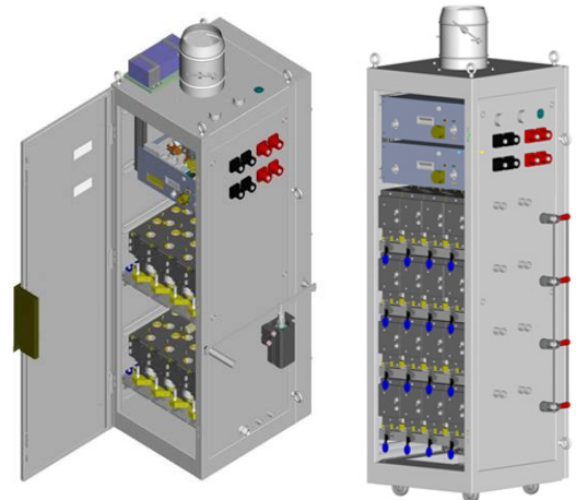
250 kW battery
